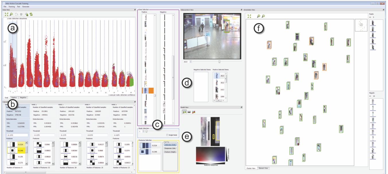
Figure 3: A screenshot of the VIAL approach by Höferlin et al. [H NH *12]. The interface is split into several interlinked areas. (a) the scatterplots for each strong classifier of the cascade; (b) detail view of each strong classifier including the respective features selected by the classifier; (c) selected instances by the user (from the scatterplots); (d) visualization of selected instances in the original video frame (context); (e) visualization of rectangle features on selected instances; (f) a 2D view for instance labeling. Reprint with permission of IEEE.
