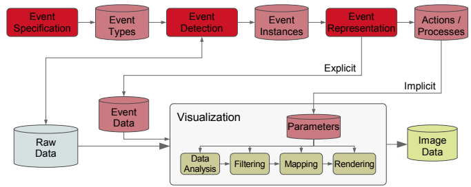
Fig. 14. Model of event-based visualization – The figure shows the major steps of event-based visualization (event specification, event detection, and event representation) attached to the well-known visualization pipeline.
